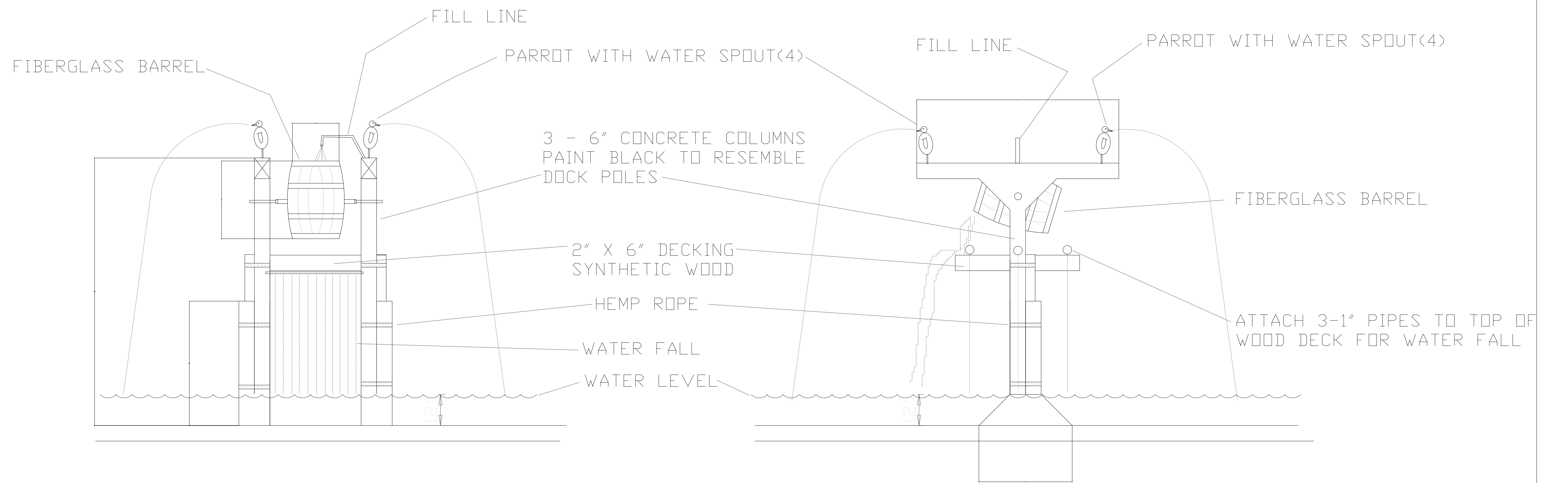
BARREL BUCKET DUMP FRONT VIEW
